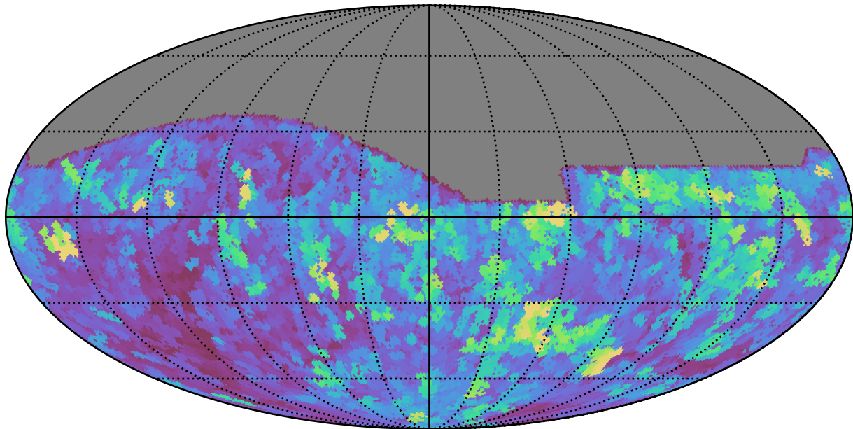
baseline_v3.3_10yrs All sky all bands: Max seeingEff
