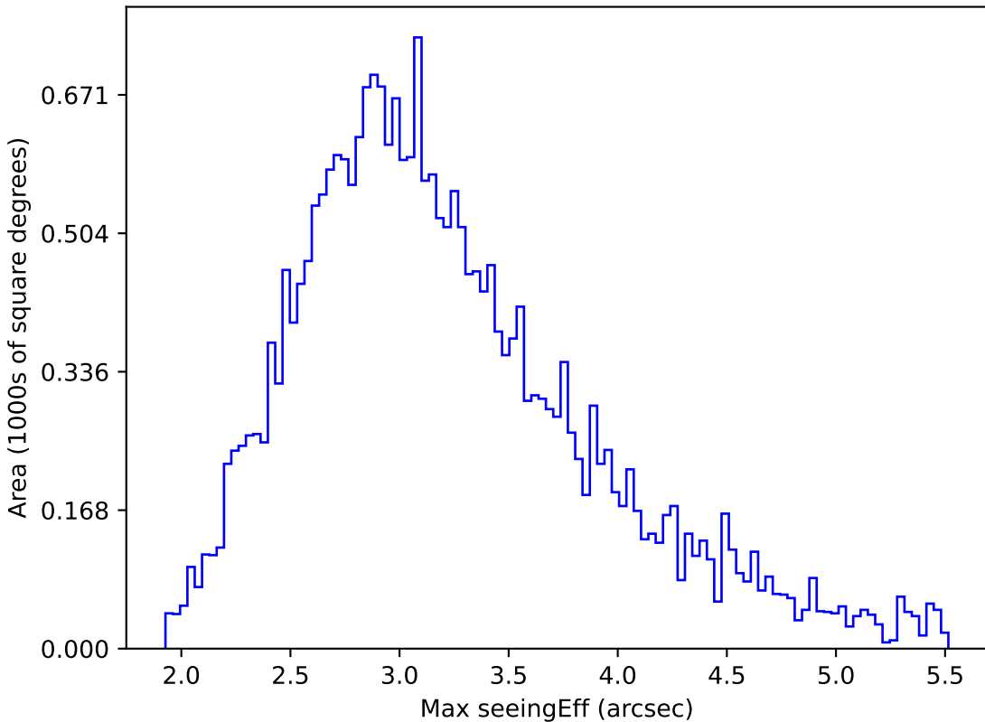
baseline_v3.3_10yrs All sky all bands: Max seeingEff
