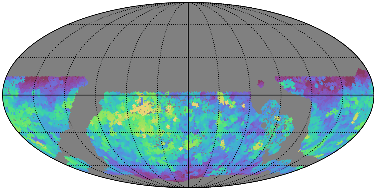
baseline_v3.3_10yrs WFD all bands: Max saturation_mag
