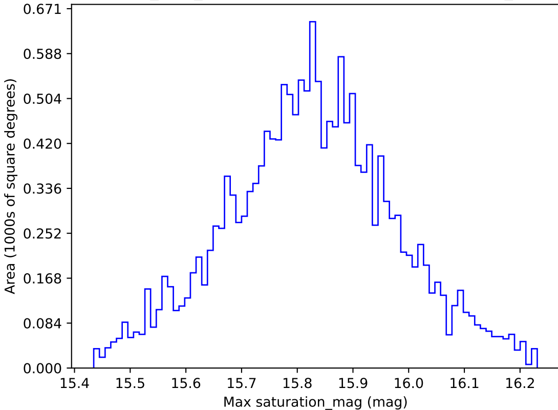
baseline_v3.3_10yrs WFD all bands: Max saturation_mag
