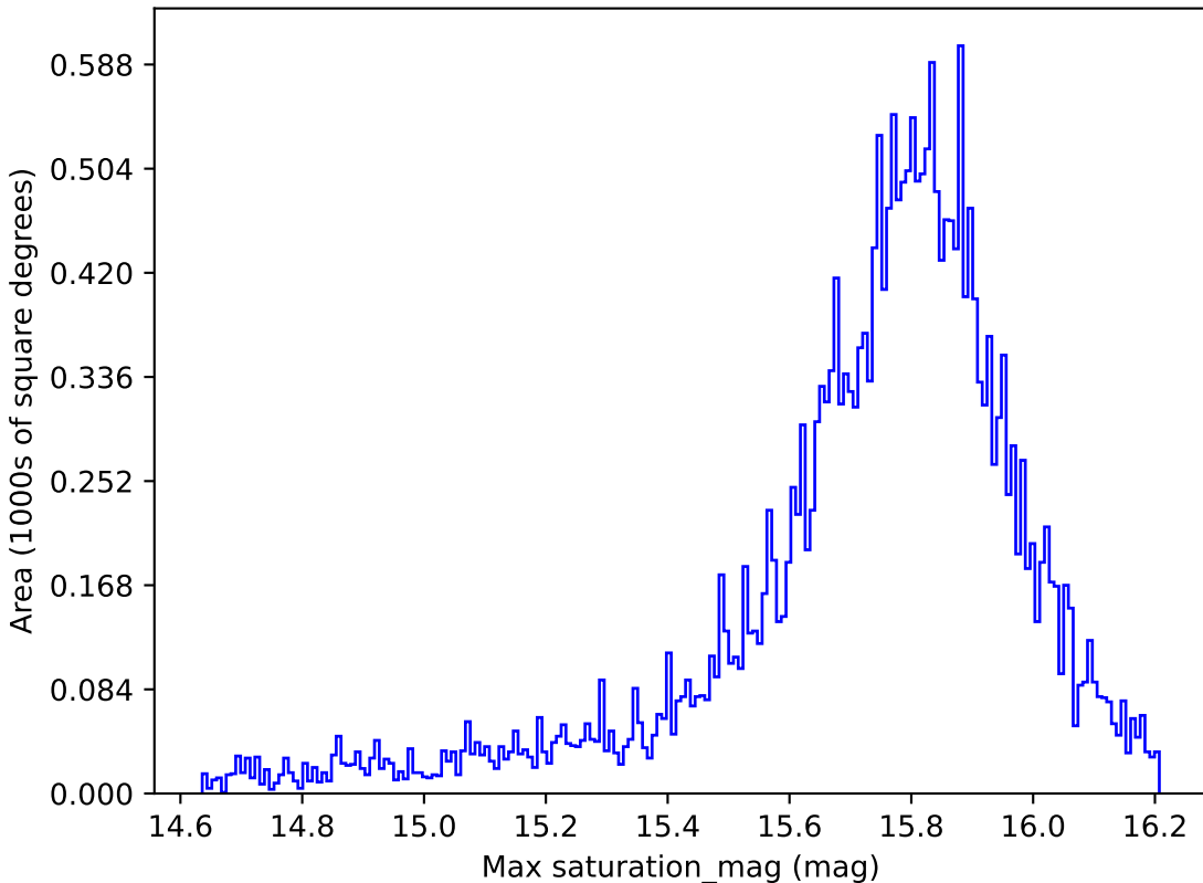
baseline_v3.3_10yrs All sky all bands: Max saturation_mag
