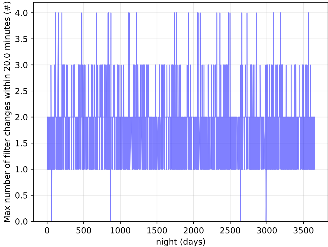
baseline_v3.3_10yrs Per Night: Max number of filter changes within 20.0 minutes
