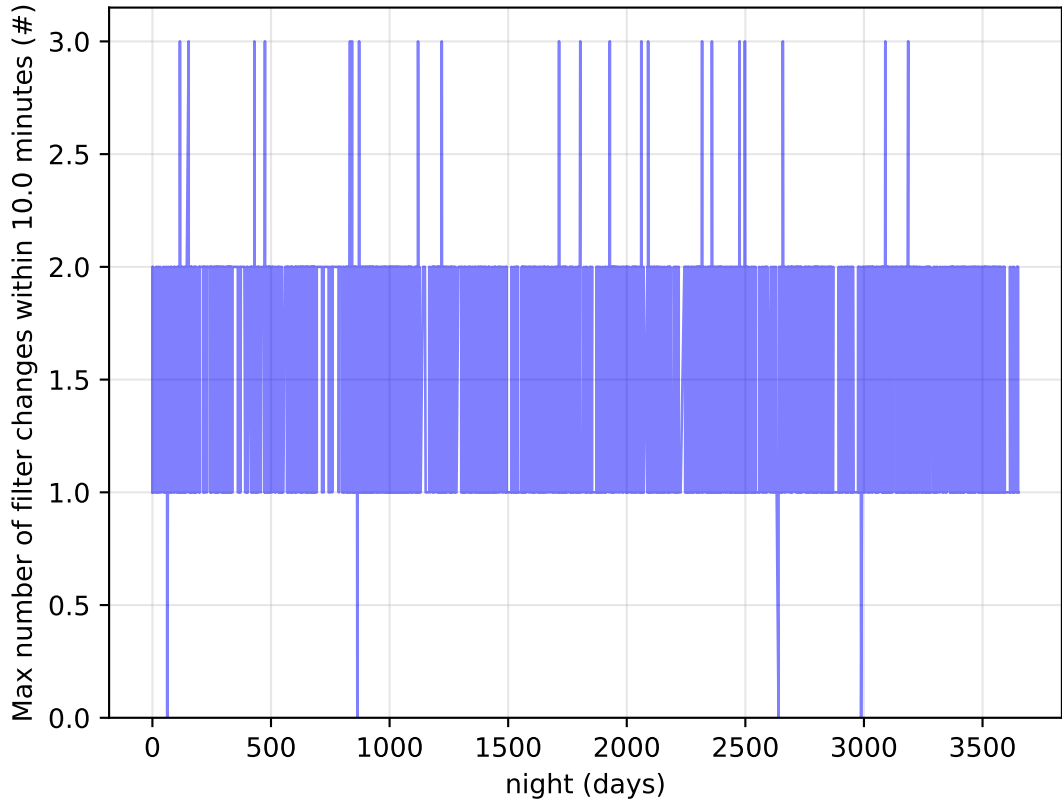
baseline_v3.3_10yrs Per Night: Max number of filter changes within 10.0 minutes
