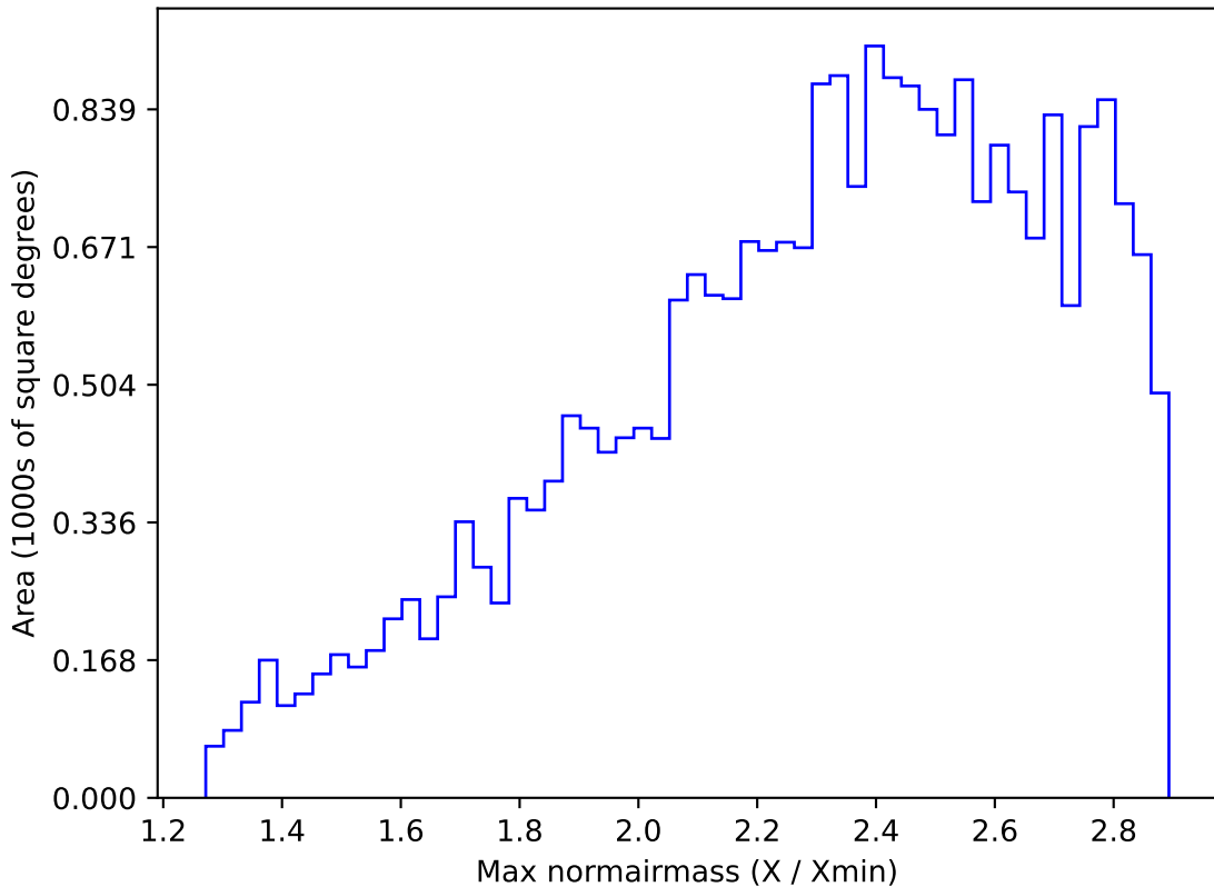
baseline_v3.3_10yrs All sky all bands: Max normairmass
