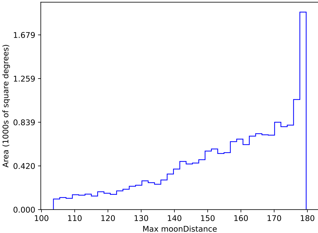
baseline_v3.3_10yrs WFD all bands: Max moonDistance
