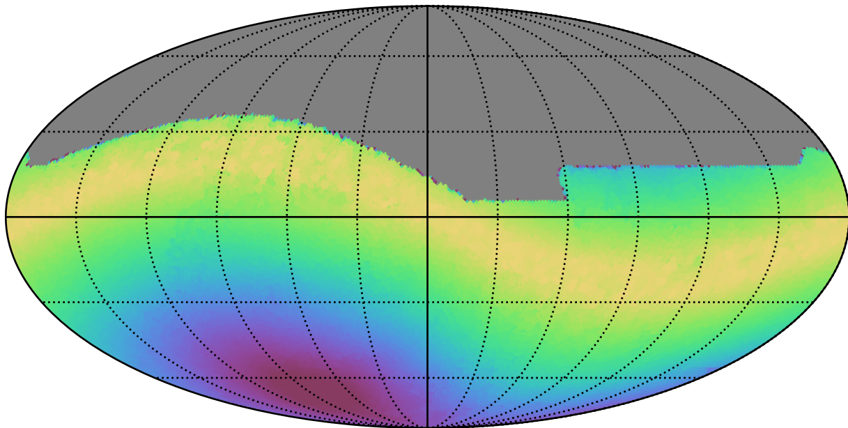
baseline_v3.3_10yrs All sky all bands: Max moonDistance
