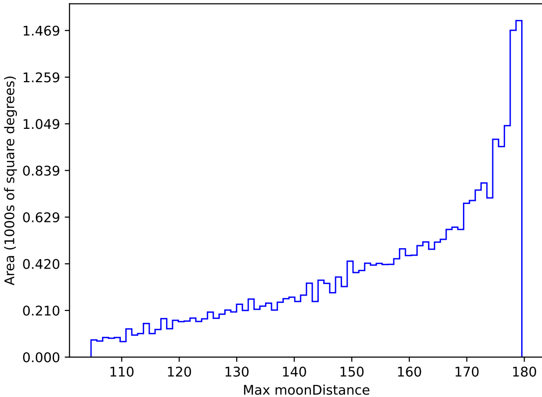
baseline_v3.3_10yrs All sky all bands: Max moonDistance
