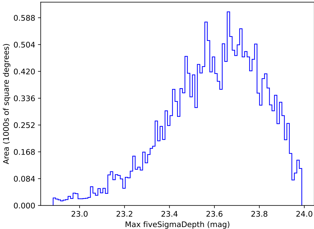
baseline_v3.3_10yrs Yr 1 u band: Max fiveSigmaDepth
