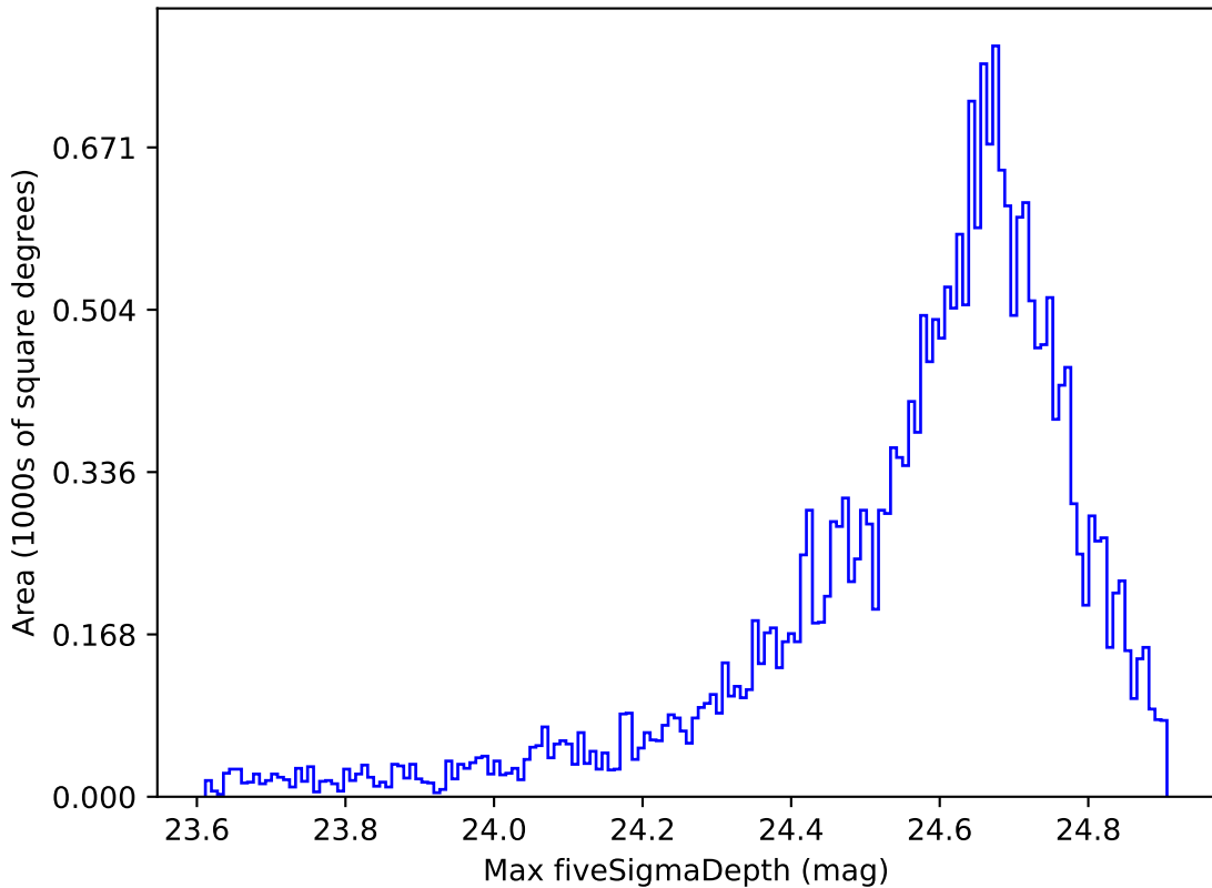
baseline_v3.3_10yrs Yr 1 r band: Max fiveSigmaDepth
