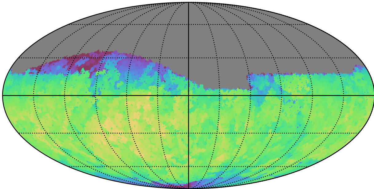
baseline_v3.3_10yrs Yr 1 i band: Max fiveSigmaDepth
