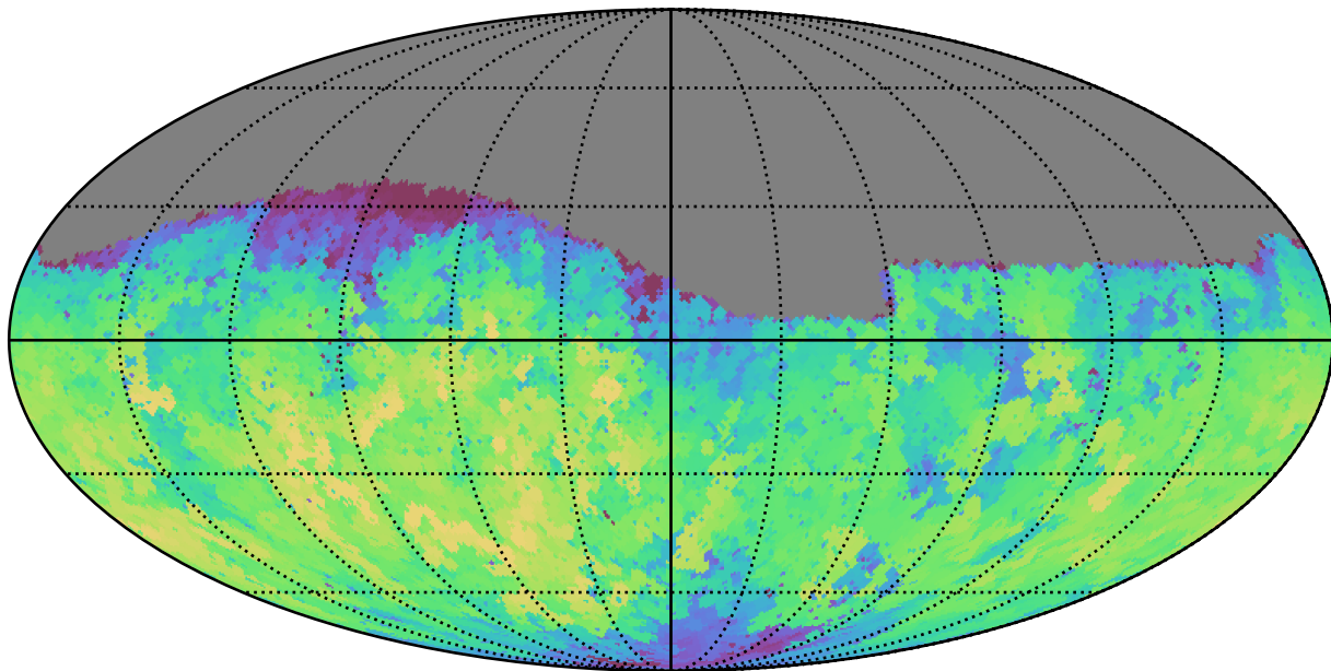
baseline_v3.3_10yrs Yr 1 g band: Max fiveSigmaDepth
