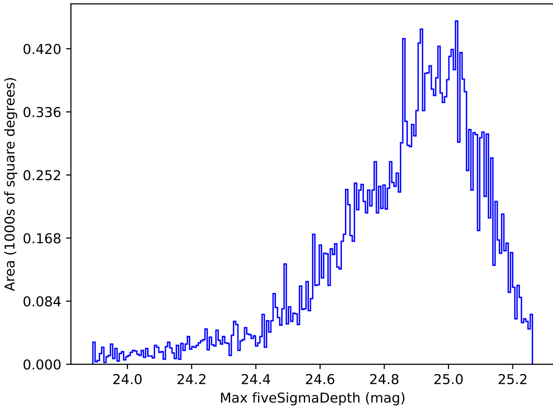
baseline_v3.3_10yrs Yr 1 all bands: Max fiveSigmaDepth
