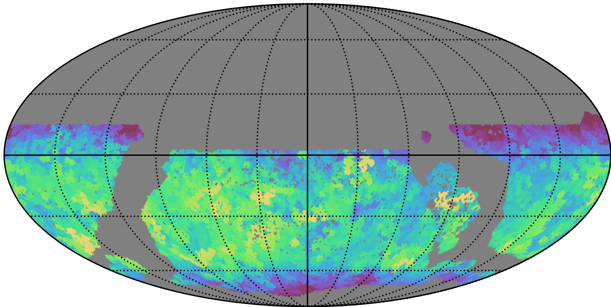
baseline_v3.3_10yrs WFD z band: Max fiveSigmaDepth
