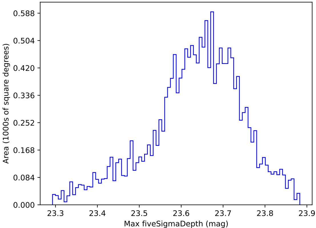
baseline_v3.3_10yrs WFD z band: Max fiveSigmaDepth
