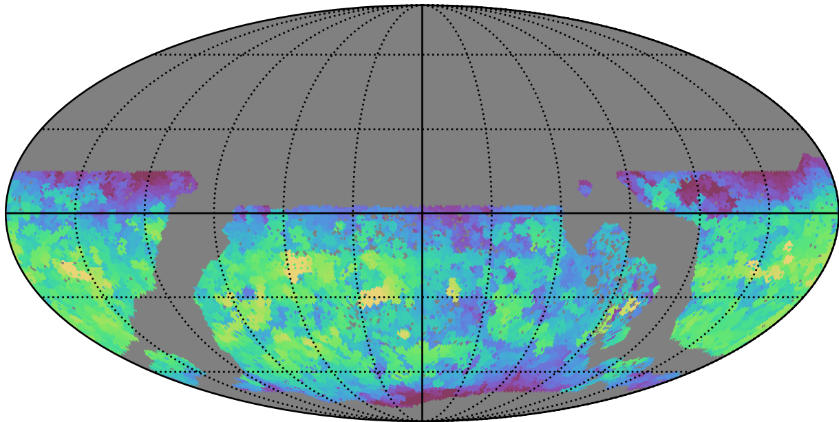
baseline_v3.3_10yrs WFD u band: Max fiveSigmaDepth
