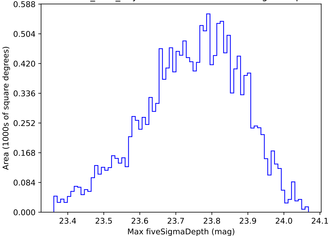
baseline_v3.3_10yrs WFD u band: Max fiveSigmaDepth
