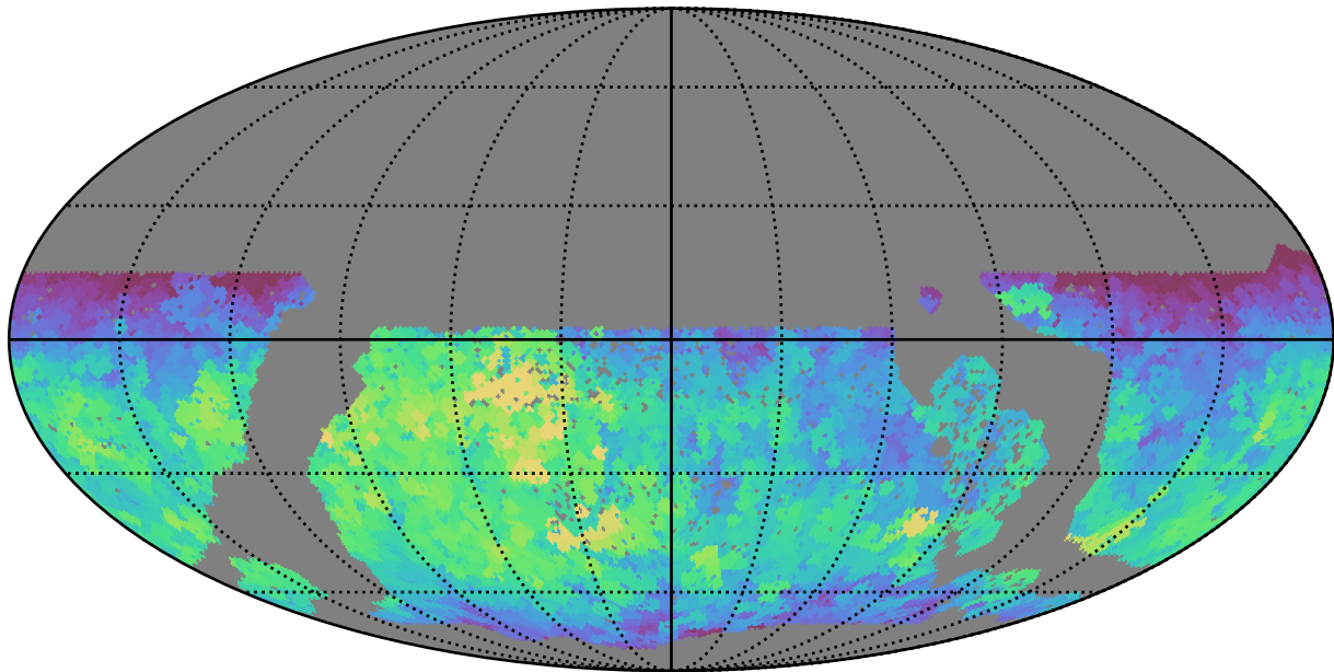
baseline_v3.3_10yrs WFD r band: Max fiveSigmaDepth
