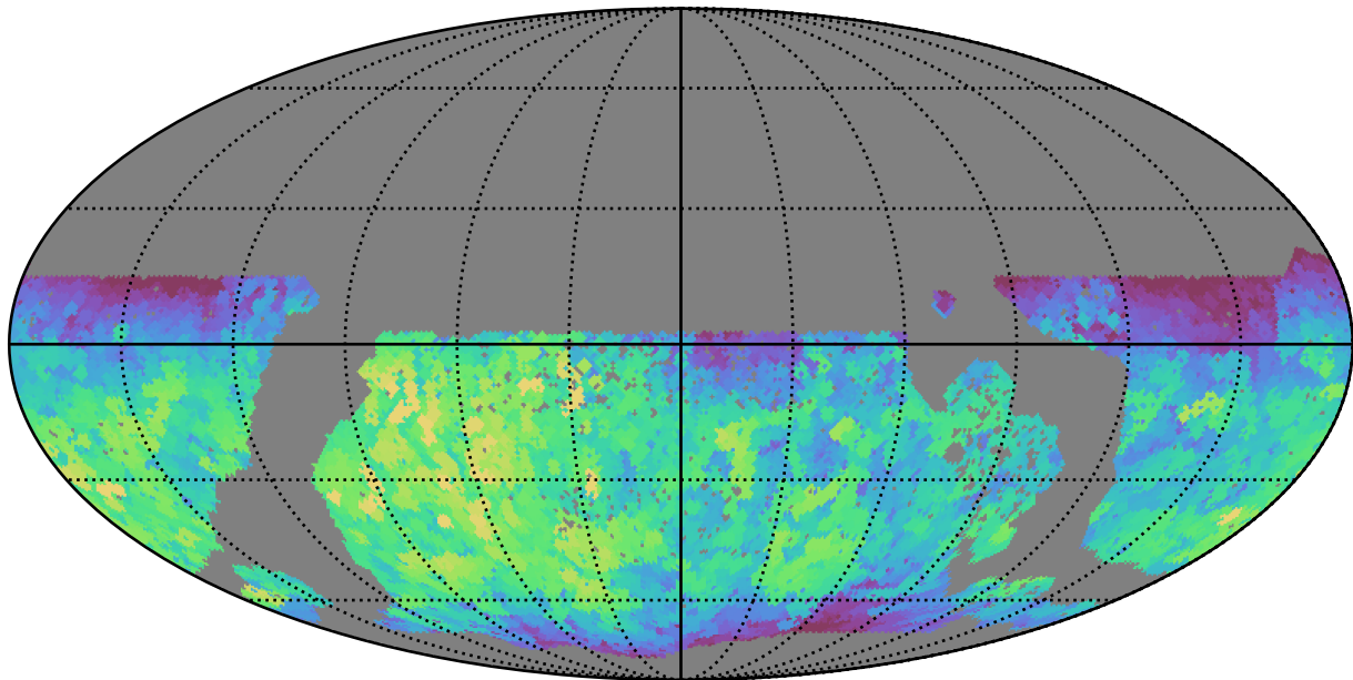
baseline_v3.3_10yrs WFD i band: Max fiveSigmaDepth
