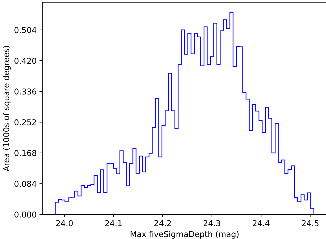
baseline_v3.3_10yrs WFD i band: Max fiveSigmaDepth
