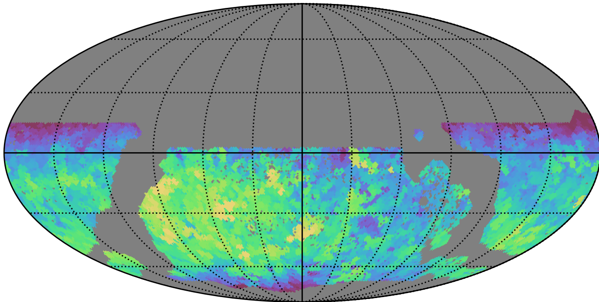
baseline_v3.3_10yrs WFD g band: Max fiveSigmaDepth
