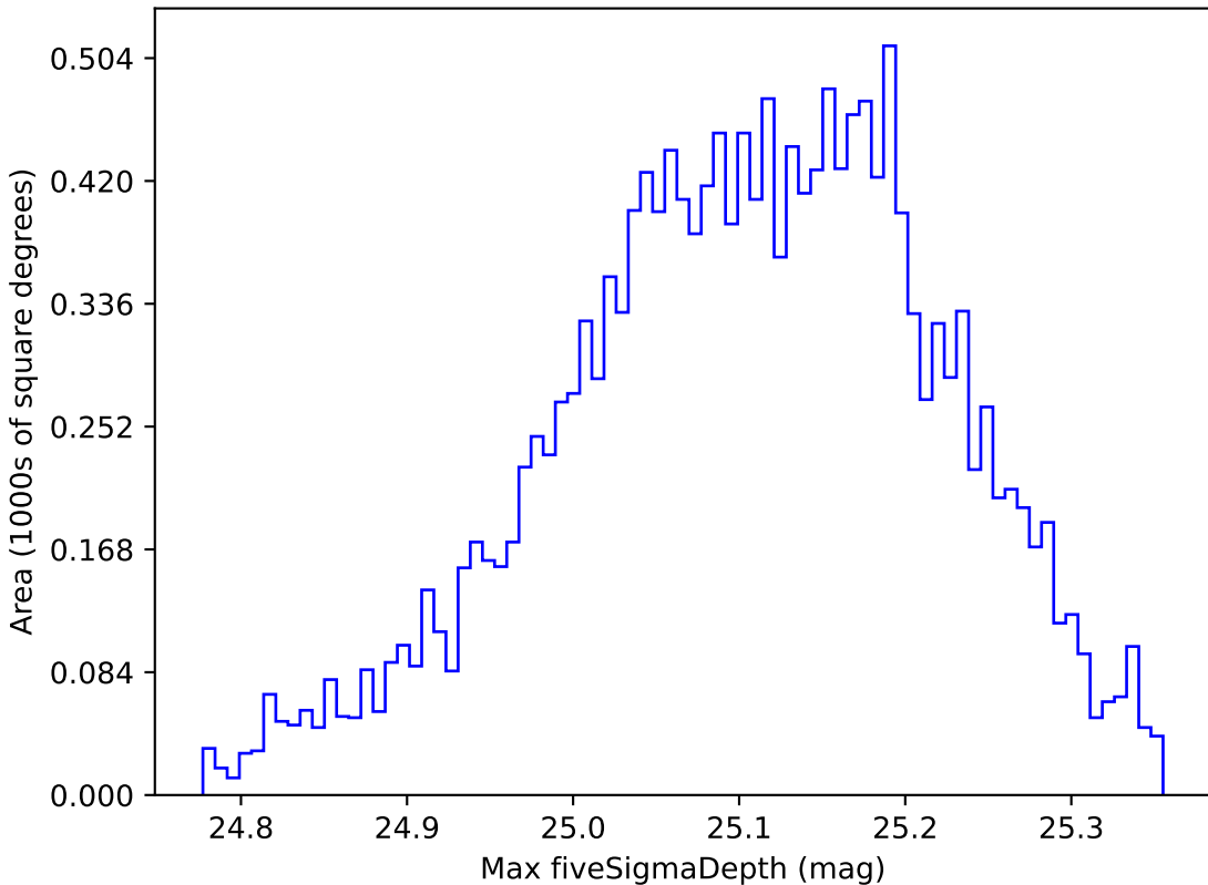
baseline_v3.3_10yrs WFD g band: Max fiveSigmaDepth
