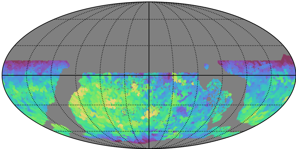
baseline_v3.3_10yrs WFD all bands: Max fiveSigmaDepth
