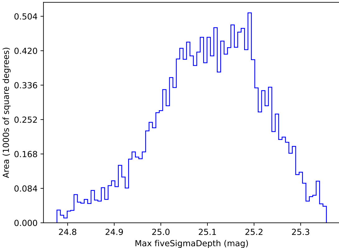
baseline_v3.3_10yrs WFD all bands: Max fiveSigmaDepth
