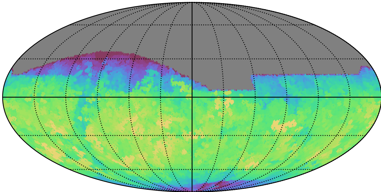
baseline_v3.3_10yrs All sky z band: Max fiveSigmaDepth
