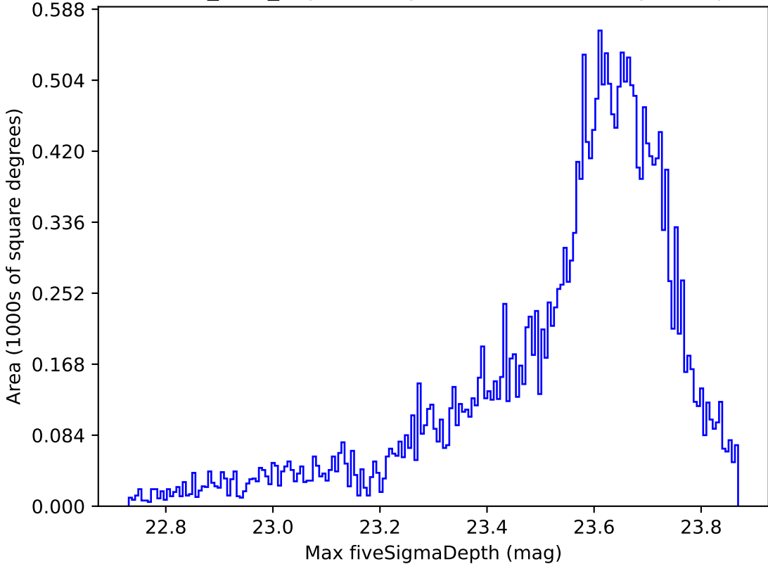
baseline_v3.3_10yrs All sky z band: Max fiveSigmaDepth
