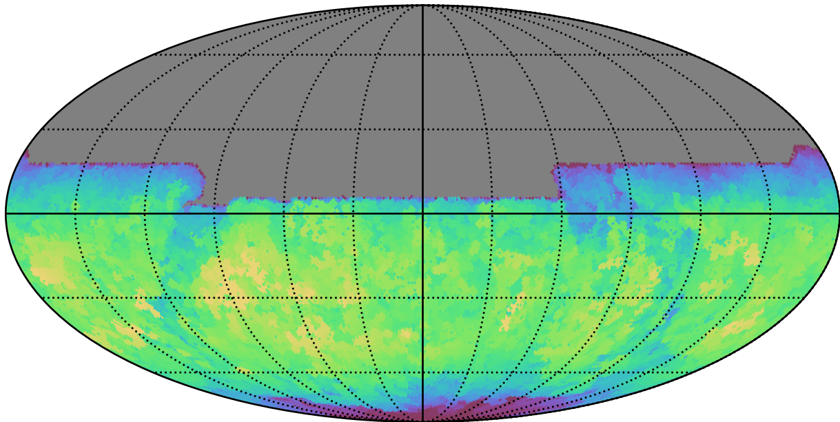
baseline_v3.3_10yrs All sky y band: Max fiveSigmaDepth
