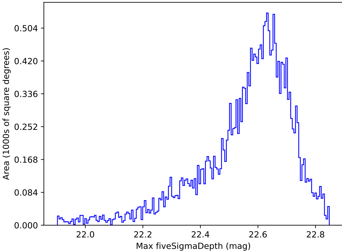
baseline_v3.3_10yrs All sky y band: Max fiveSigmaDepth
