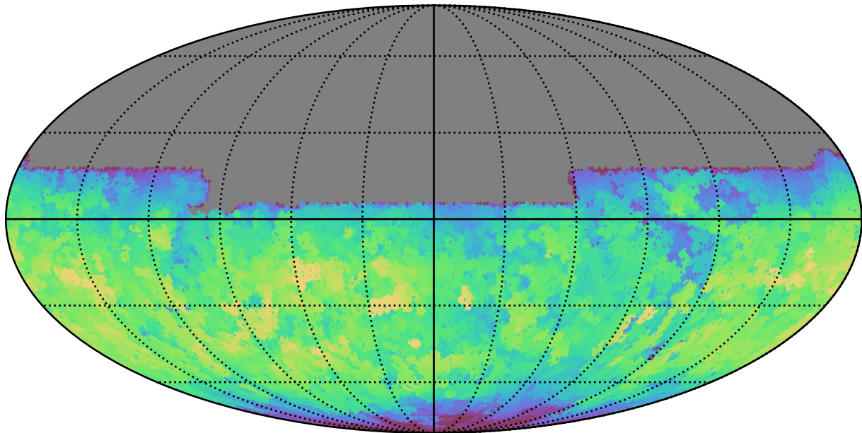
baseline_v3.3_10yrs All sky u band: Max fiveSigmaDepth
