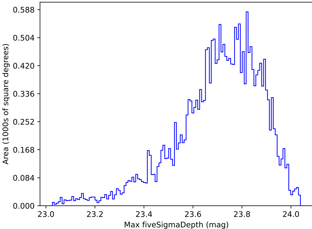
baseline_v3.3_10yrs All sky u band: Max fiveSigmaDepth
