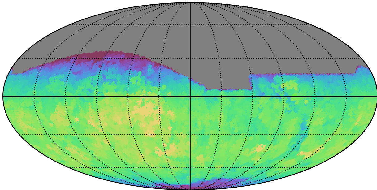
baseline_v3.3_10yrs All sky r band: Max fiveSigmaDepth
