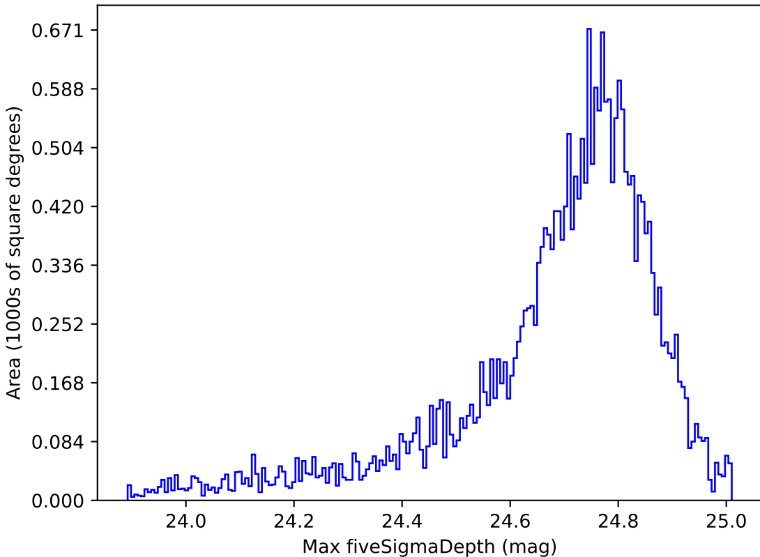
baseline_v3.3_10yrs All sky r band: Max fiveSigmaDepth
