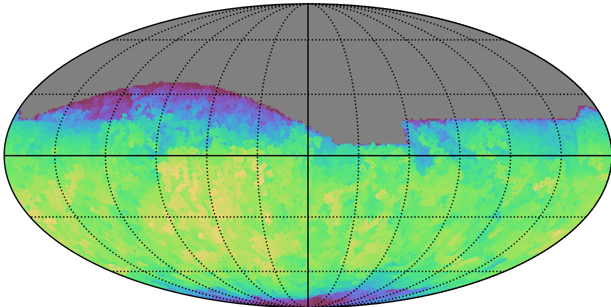
baseline_v3.3_10yrs All sky i band: Max fiveSigmaDepth
