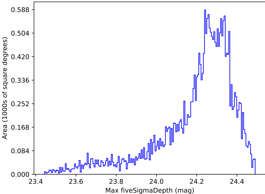
baseline_v3.3_10yrs All sky i band: Max fiveSigmaDepth
