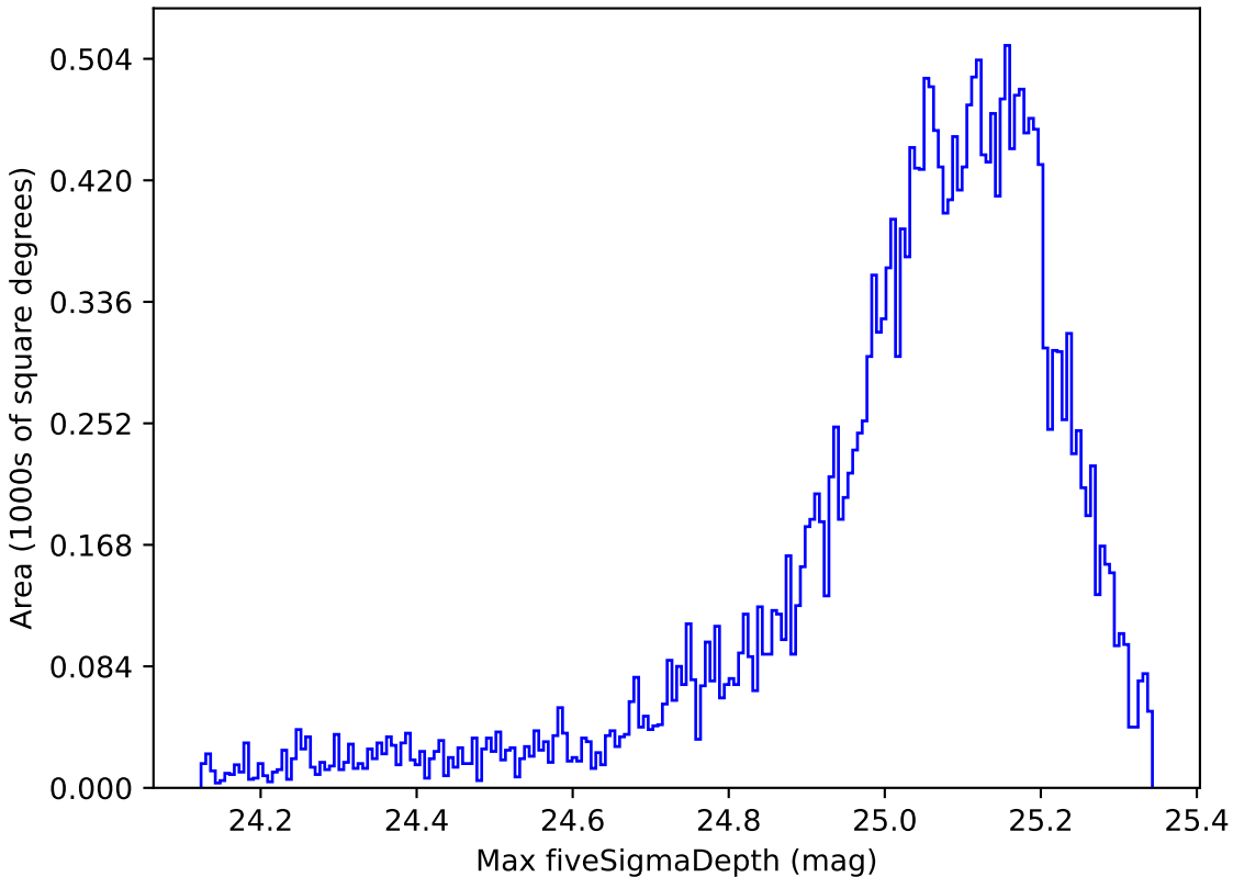
baseline_v3.3_10yrs All sky g band: Max fiveSigmaDepth
