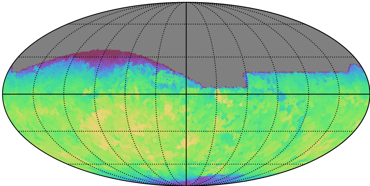
baseline_v3.3_10yrs All sky all bands: Max fiveSigmaDepth
