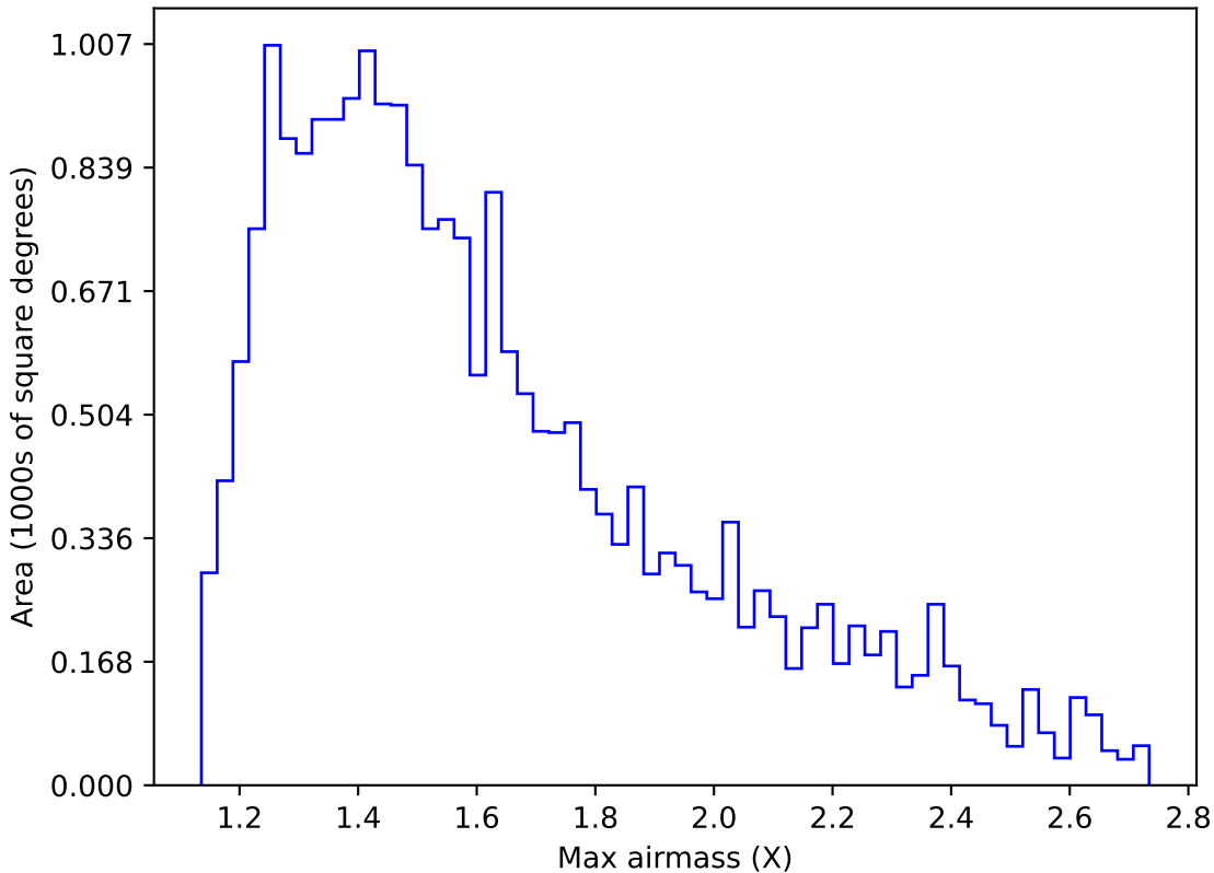
baseline_v3.3_10yrs Yr 1 y band: Max airmass
