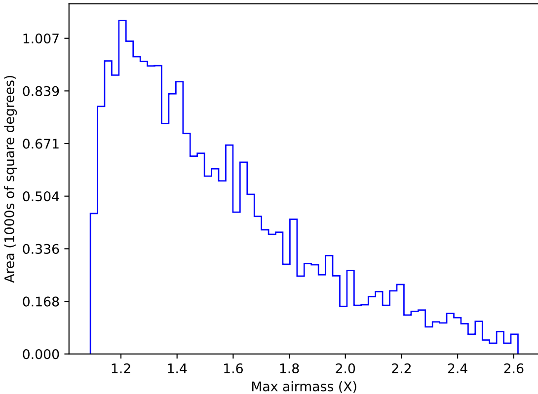
baseline_v3.3_10yrs Yr 1 u band: Max airmass
