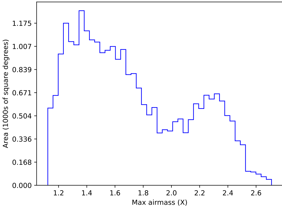
baseline_v3.3_10yrs Yr 1 r band: Max airmass
