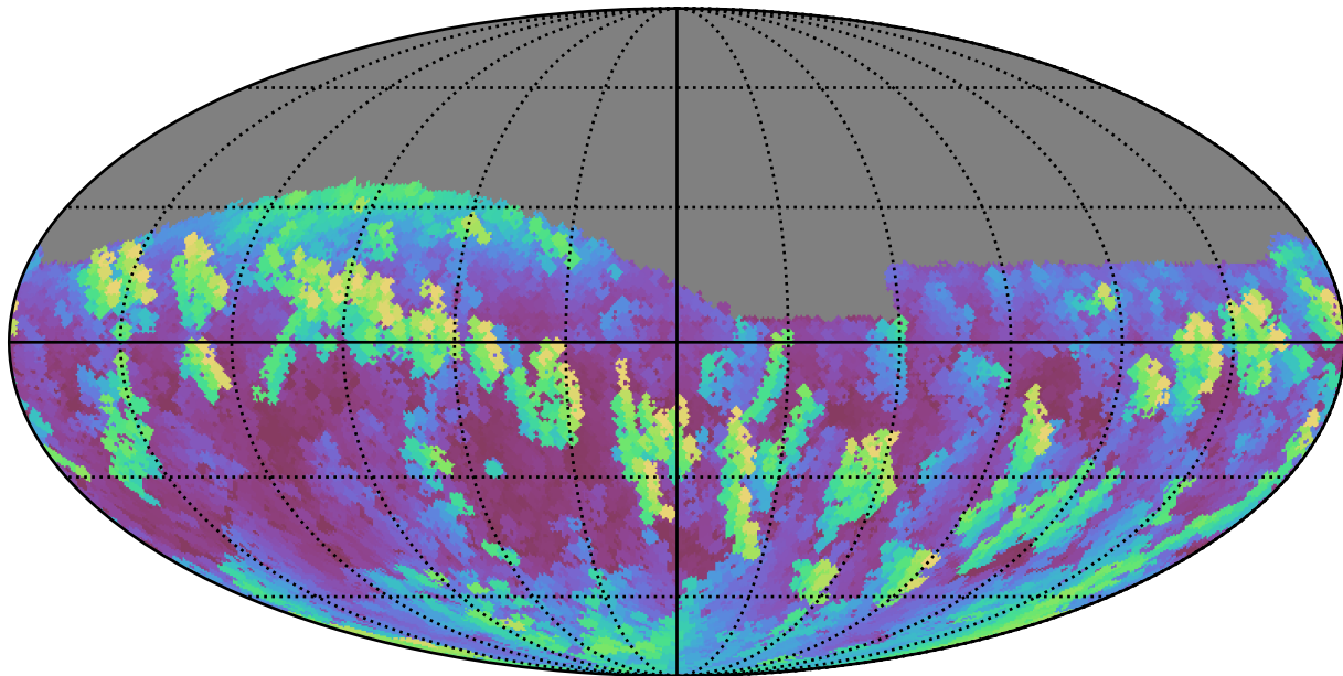
baseline_v3.3_10yrs Yr 1 i band: Max airmass
