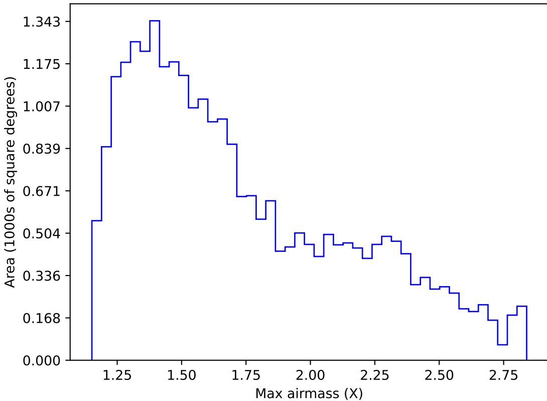
baseline_v3.3_10yrs Yr 1 i band: Max airmass
