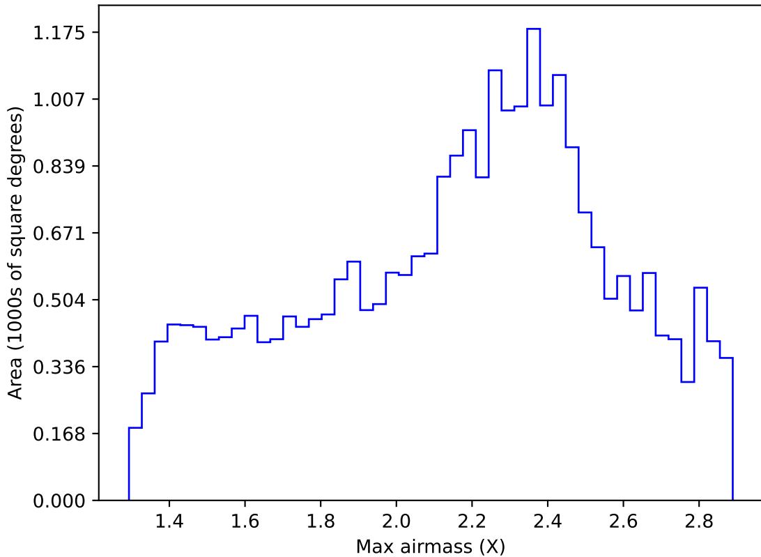
baseline_v3.3_10yrs Yr 1 all bands: Max airmass
