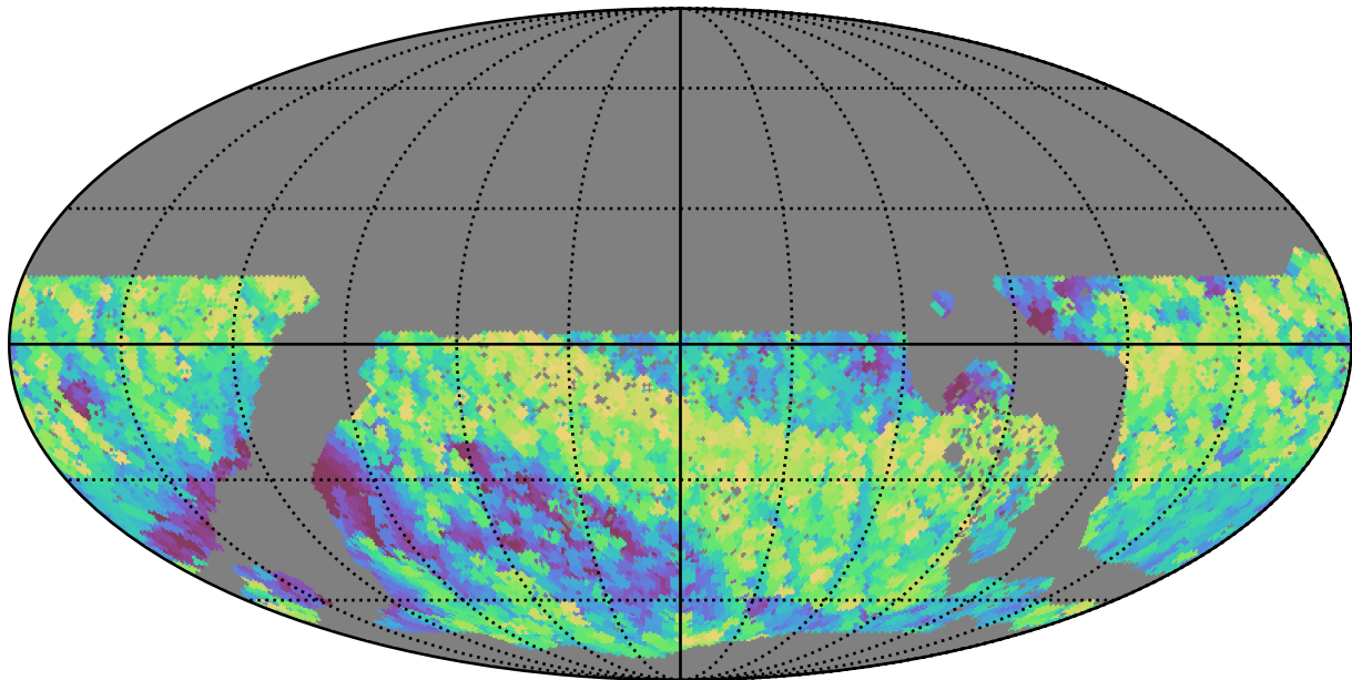
baseline_v3.3_10yrs WFD z band: Max airmass
