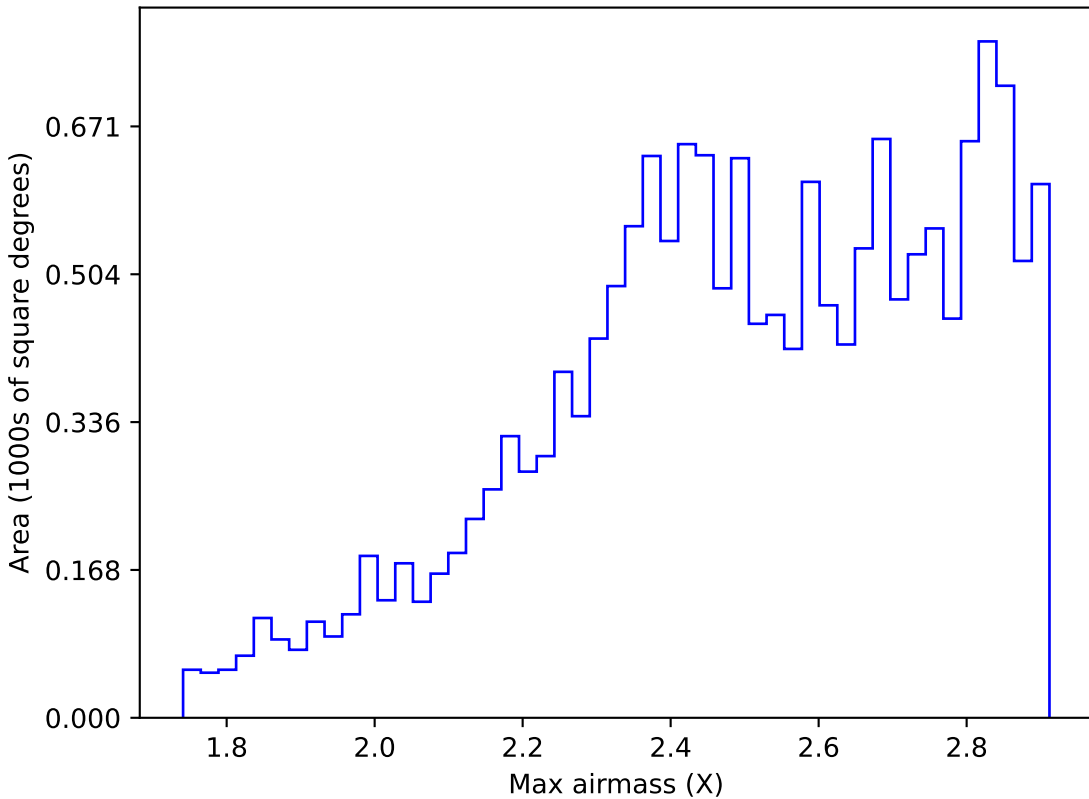
baseline_v3.3_10yrs WFD z band: Max airmass
