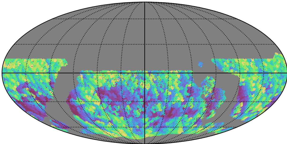
baseline_v3.3_10yrs WFD y band: Max airmass
