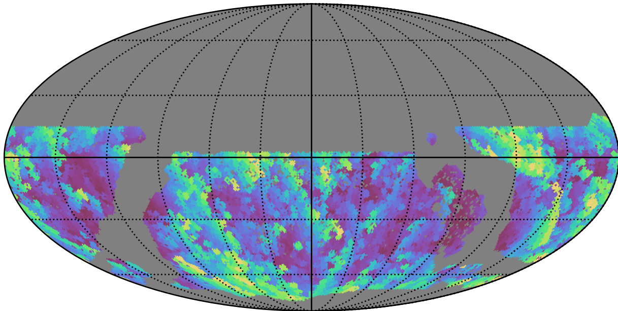
baseline_v3.3_10yrs WFD u band: Max airmass
