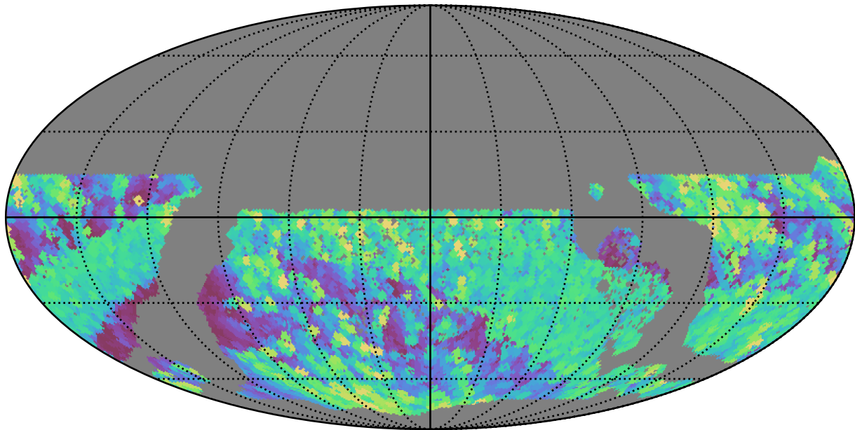
baseline_v3.3_10yrs WFD r band: Max airmass
